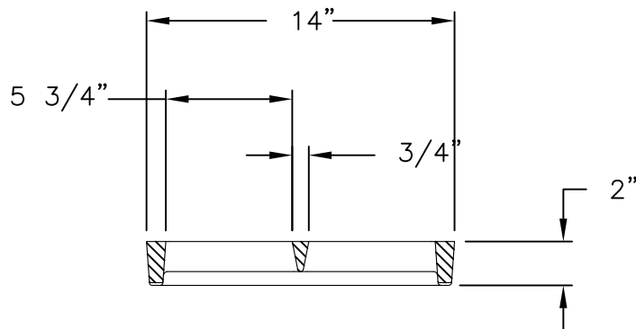
GRATE SECTION
